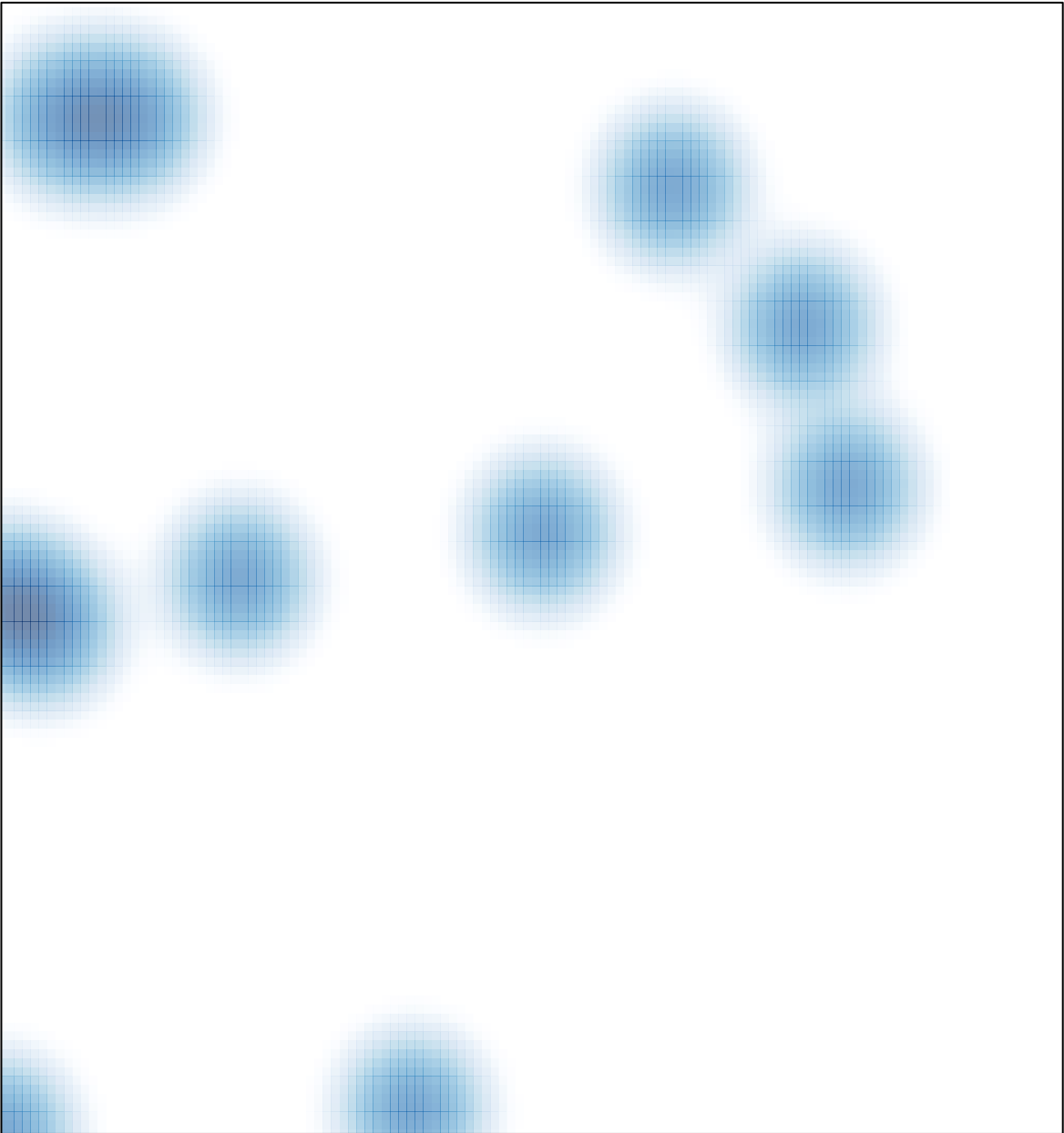
# features = 16 , max = 2
